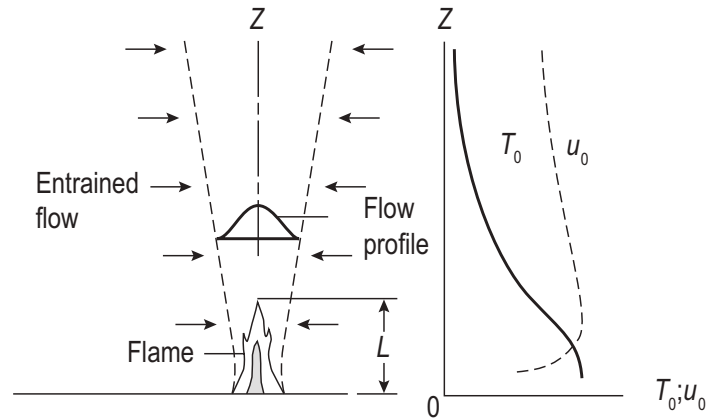
Features of a Turbulent Fire Plume, Including Axial Variations on the Centerline of Mean Excess Temperature, \Delta T_0 , and Mean Velocity, u_0
